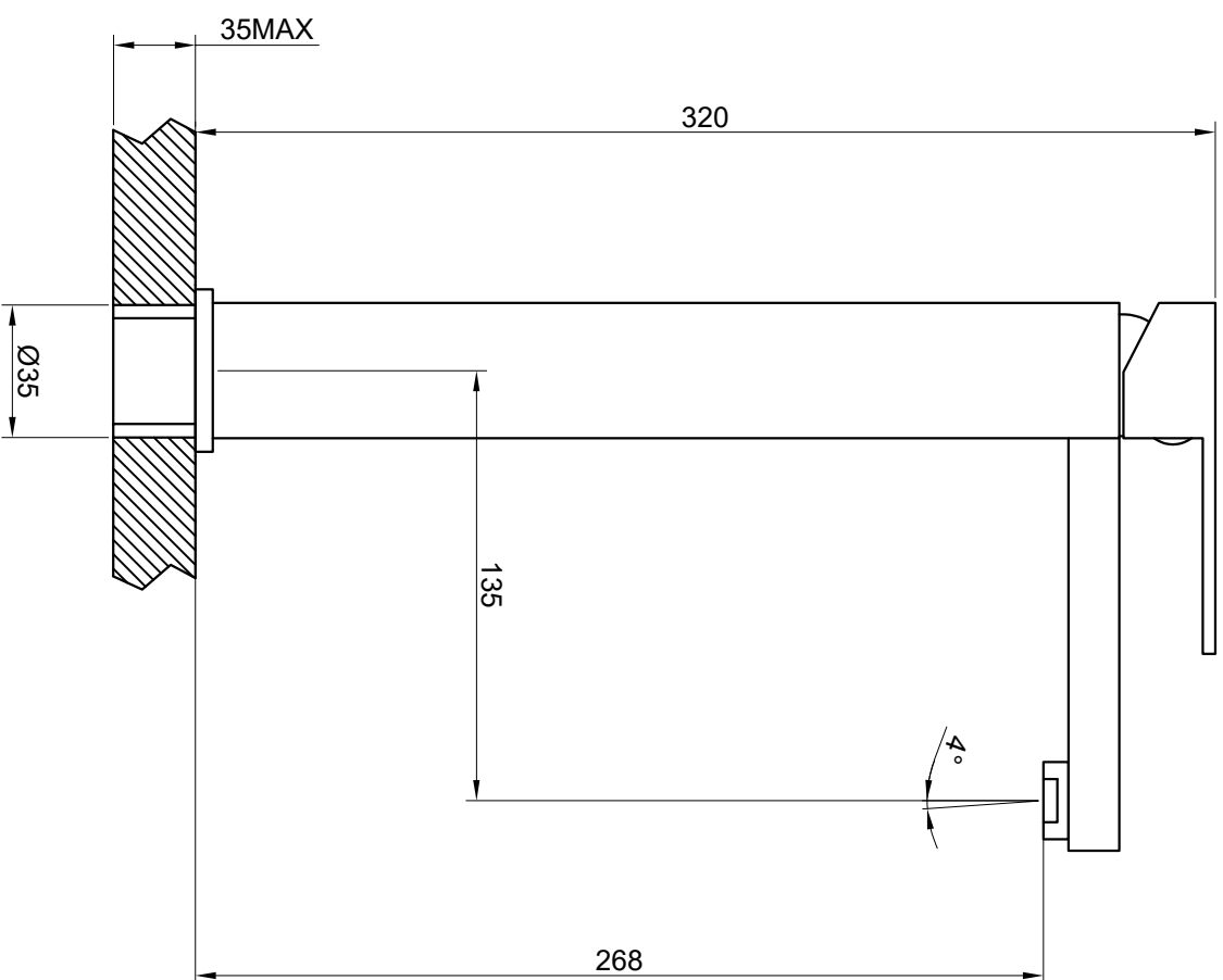
BP70- Single-Lever Tail W/HB Mixer
